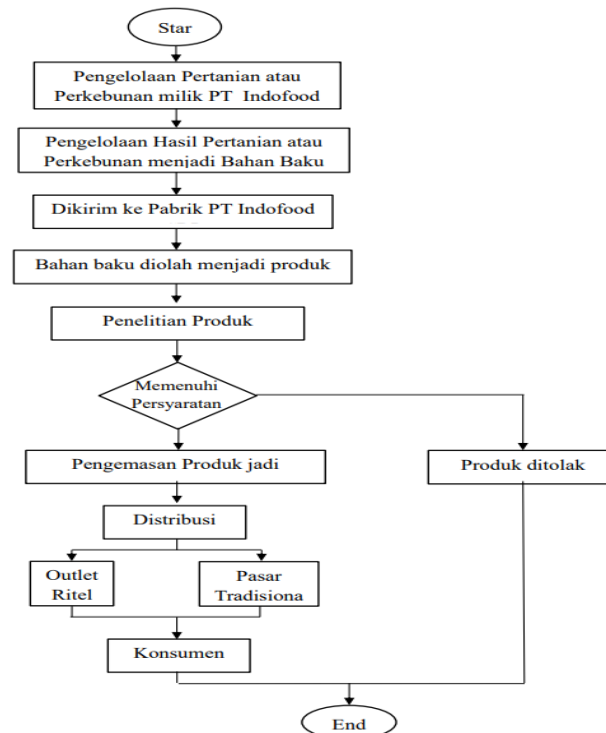
Fig 3. Flowchart Activity
