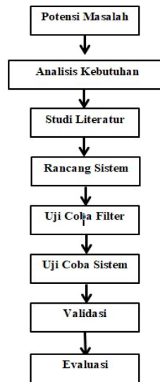
Gambar 2. Prosedur Penelitian
